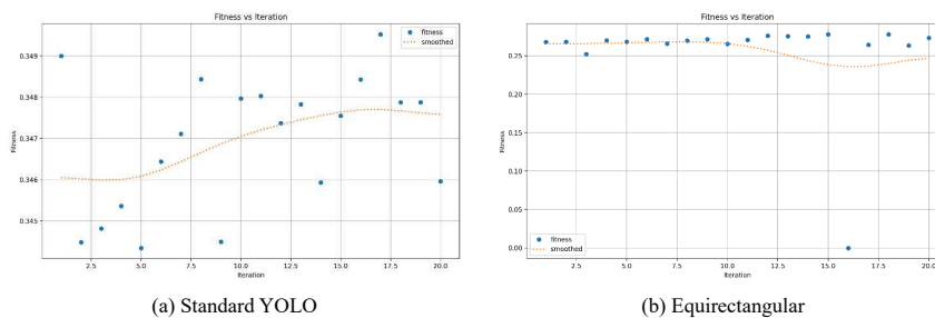
Fig. 2: Tune Fitness Comparison
