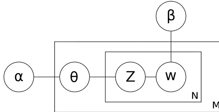
Fig. 1. LDA Diagram
