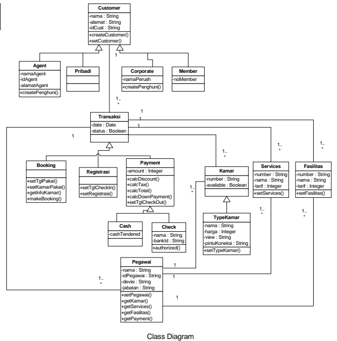
Class Diagram
