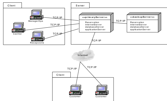
Gambar 10. Gambaran diagram deployment studi kasus
