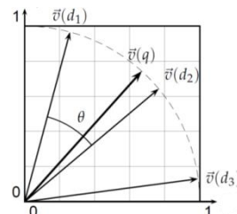
Gambar 3. Representasi vector space models
