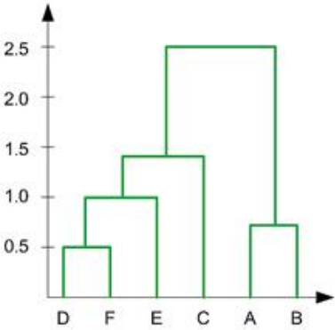
Gambar 5. Contoh Dendogram
