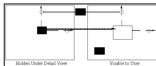
Gambar 7. Bifocal Browser
