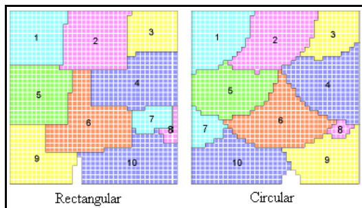
Gambar 10. Algoritma Bubblemaps
