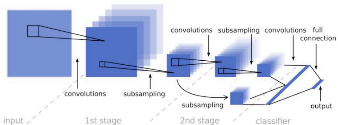
Gambar 1. Arsitektur Convolutional Neural Network (CNN) [15].
