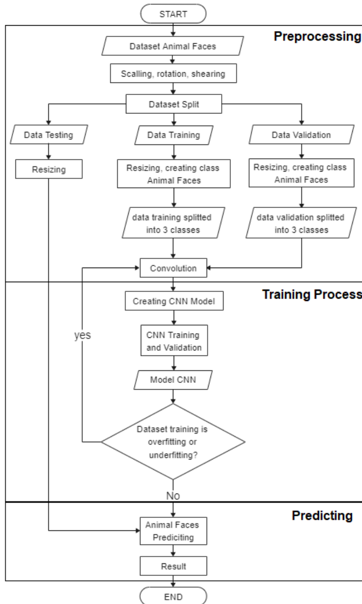
Gambar 2. Flowchart penelitian.
